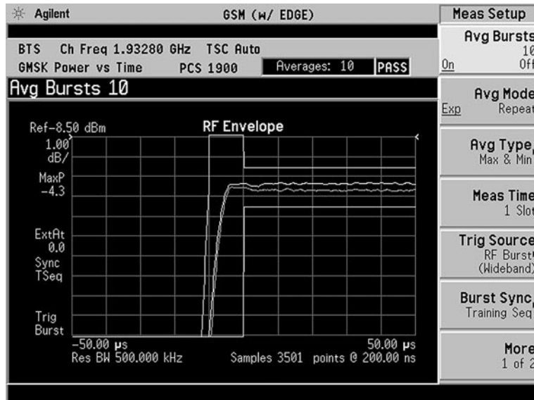
Figure 14. Rising edge of GSM burst with averaging on
