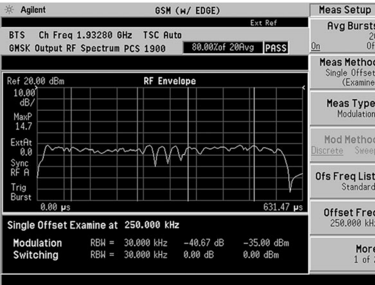
Figure 26. ORFS spectrum due to modulation at 250 kHz
