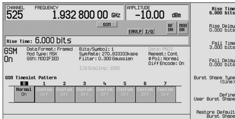
Figure 15. Modified burst shape
