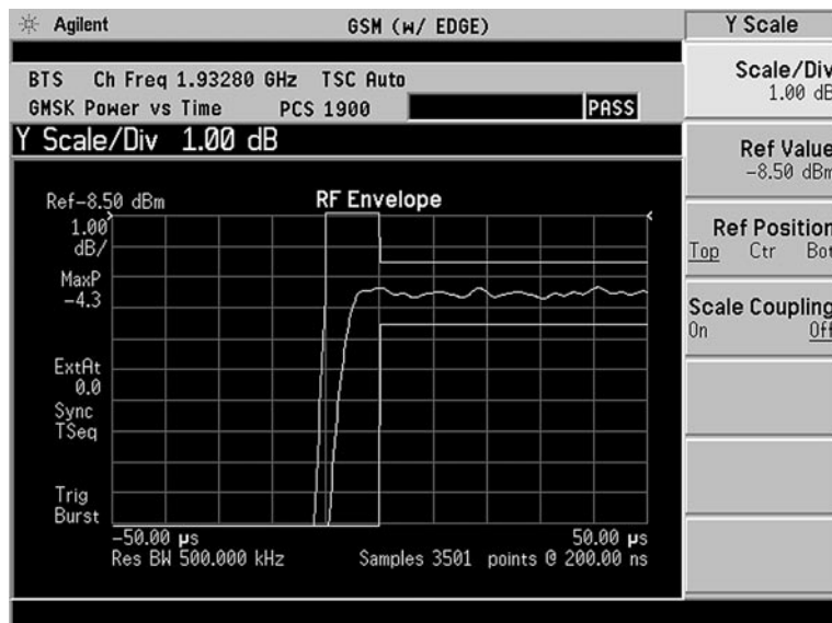
Figure 13. GSM power versus time measurement rising edge of burst
