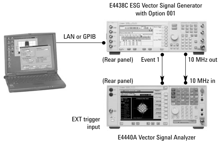
Figure 1. Demo set-up
