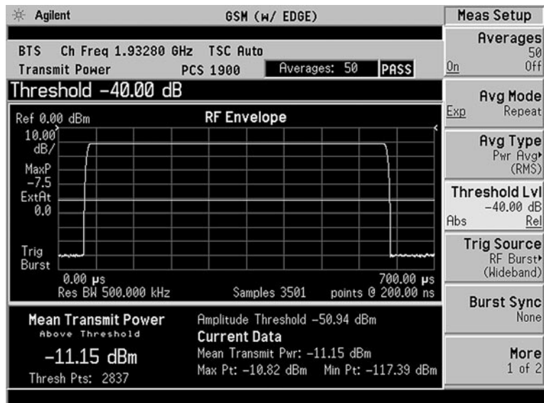
Figure 11. Transmit power measurement
