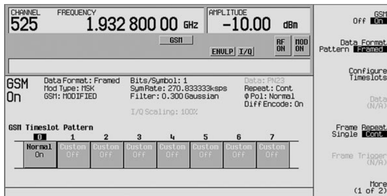
Figure 5. GSM main menu page 1
