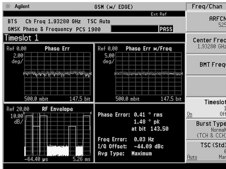
Figure 19. Phase and frequency error
