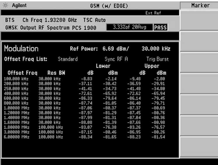
Figure 25. ORFS spectrum due to modulation
