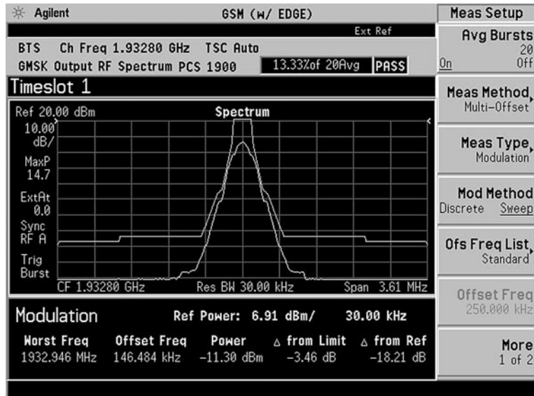
Figure 27. ORFS with mask GMSK Tx band spurious
