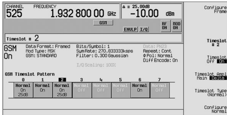
Figure 17. GSM alternate timeslot setting
