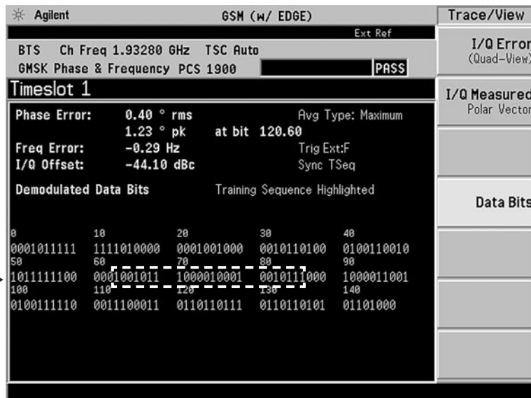
Figure 23. I and Q demodulated bits
