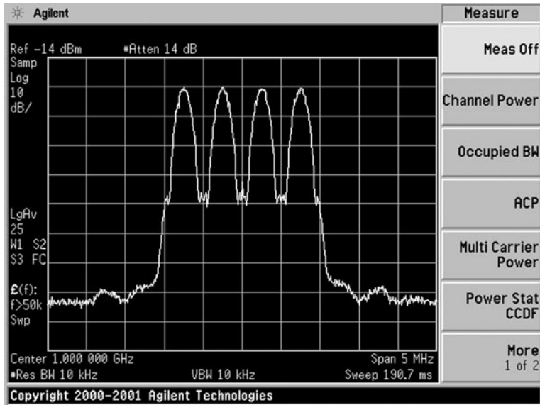
Figure 37. Spectrum of 4 EDGE modulated carriers spaced 500 kHz apart
