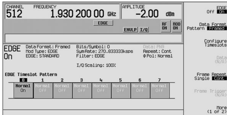
Figure 30. EDGE main menu page 1
