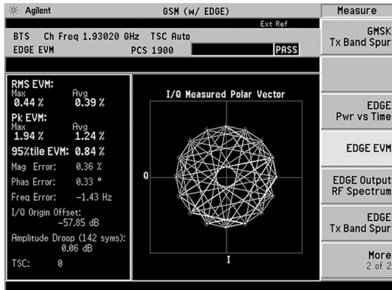
Figure 33. EDGE polar vector plot
