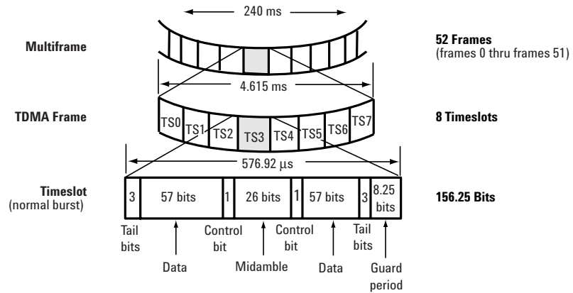
Figure 9. GSM burst with packets mapped onto a PDTCH
