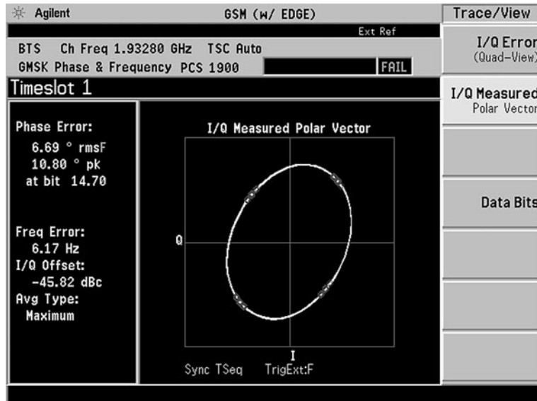
Figure 22. I/Q polar vector plot of impaired GSM signal
