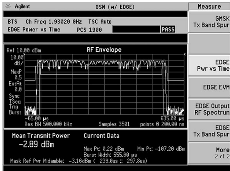
Figure 32. EDGE power versus time
