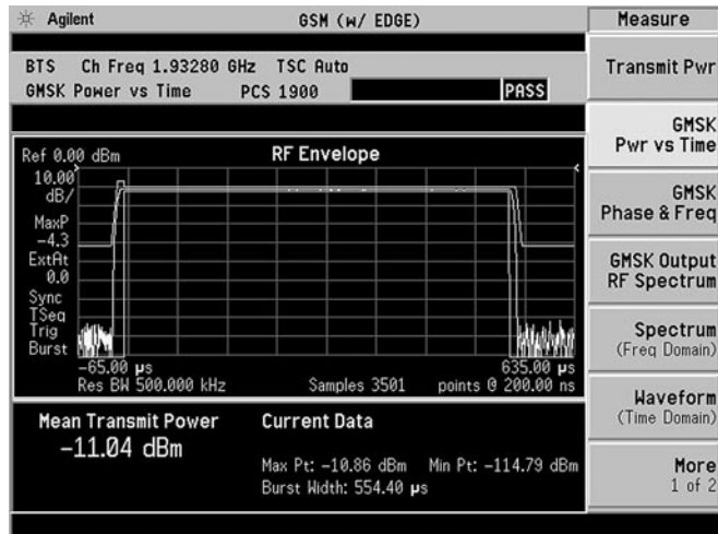
Figure 12. GSM power versus time measurement
