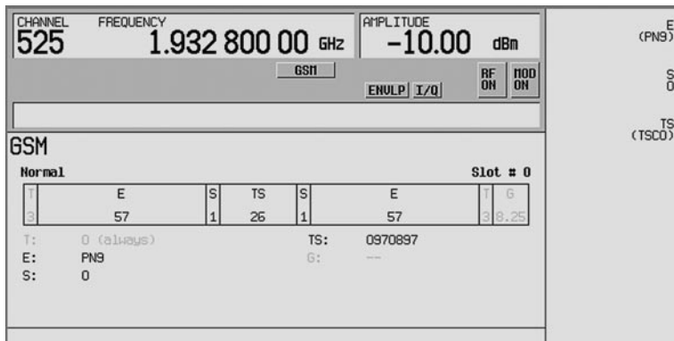
Figure 8. GSM configure one timeslot
