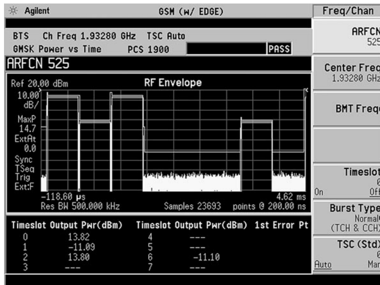
Figure 18. Multi-slot power versus time
