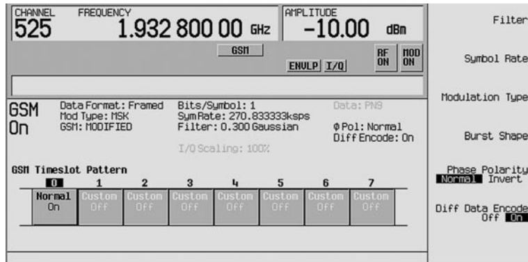
Figure 6. GSM modify standard submenu
