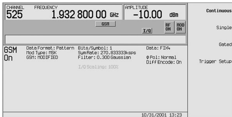
Figure 3. GSM pattern trigger menu
