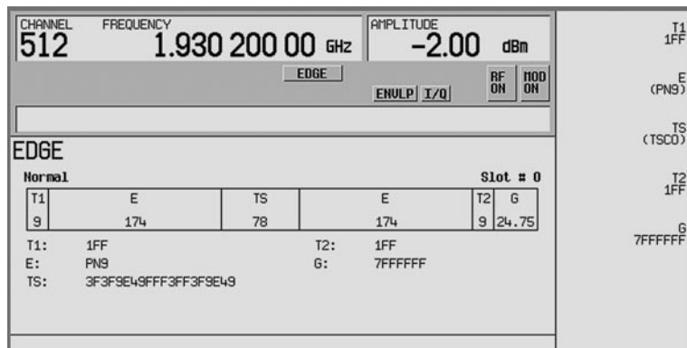
Figure 31. EDGE Normal Burst Configure Timeslot menu
