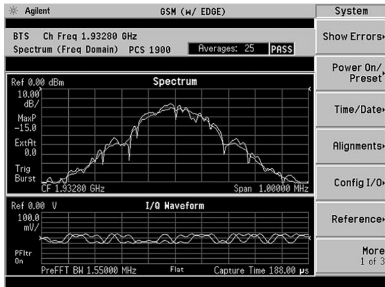
Figure 10. GSM spectrum and I/Q waveforms
