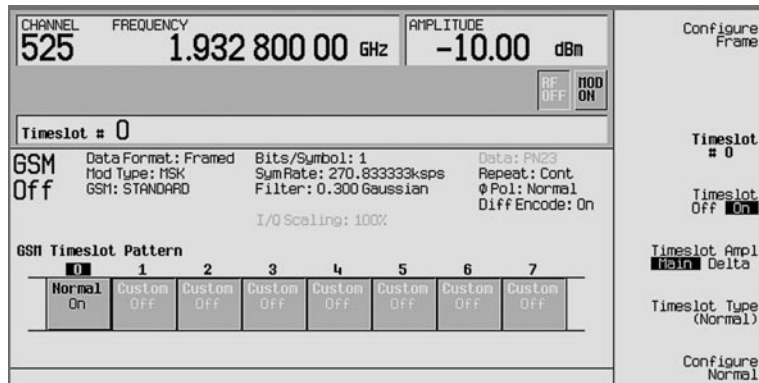
Figure 7. GSM configure timeslot menu
