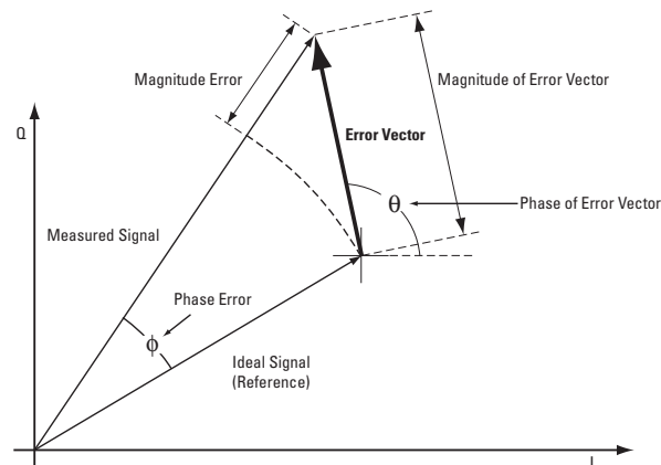
Figure 29. The error vector diagram
