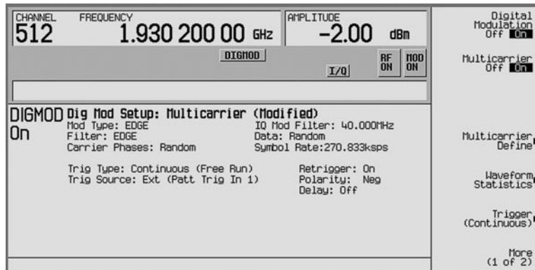
Figure 35. Digital Modulation menu for creating a multicarrier EDGE modulated waveform
