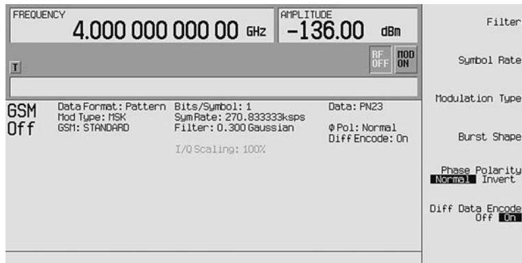
Figure 4b. Modify standard submenu
