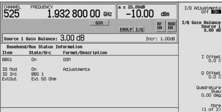
Figure 21. Added I/Q impairments to the GSM signal
