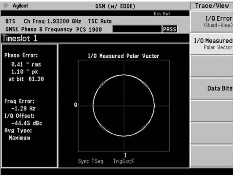
Figure 20. I/Q polar vector plot
