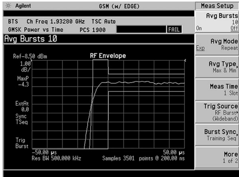
Figure 16. Modified GSM burst failing transmit spectral mask measurement
