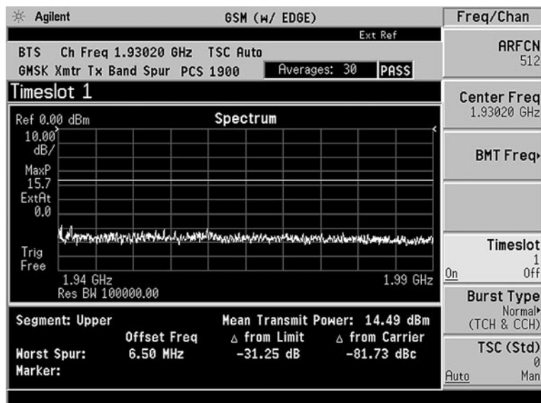
Figure 28. GMSK Tx band spurious
