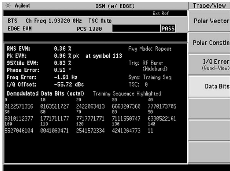
Figure 34. EDGE demodulated data bits
